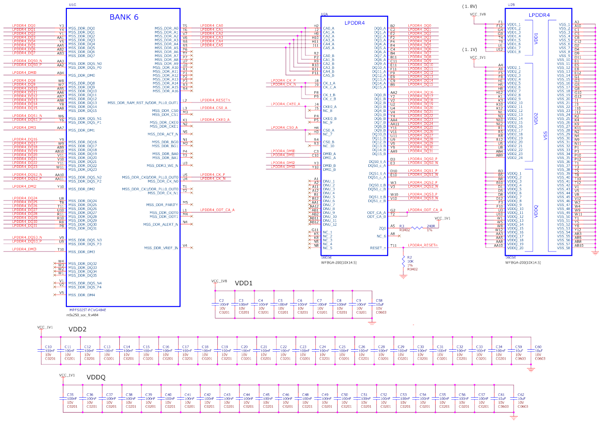
Fig. 3.29: LPDDR4 memory
