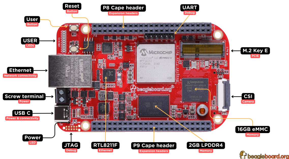
Fig. 1.1: BeagleV-Fire board front components location
